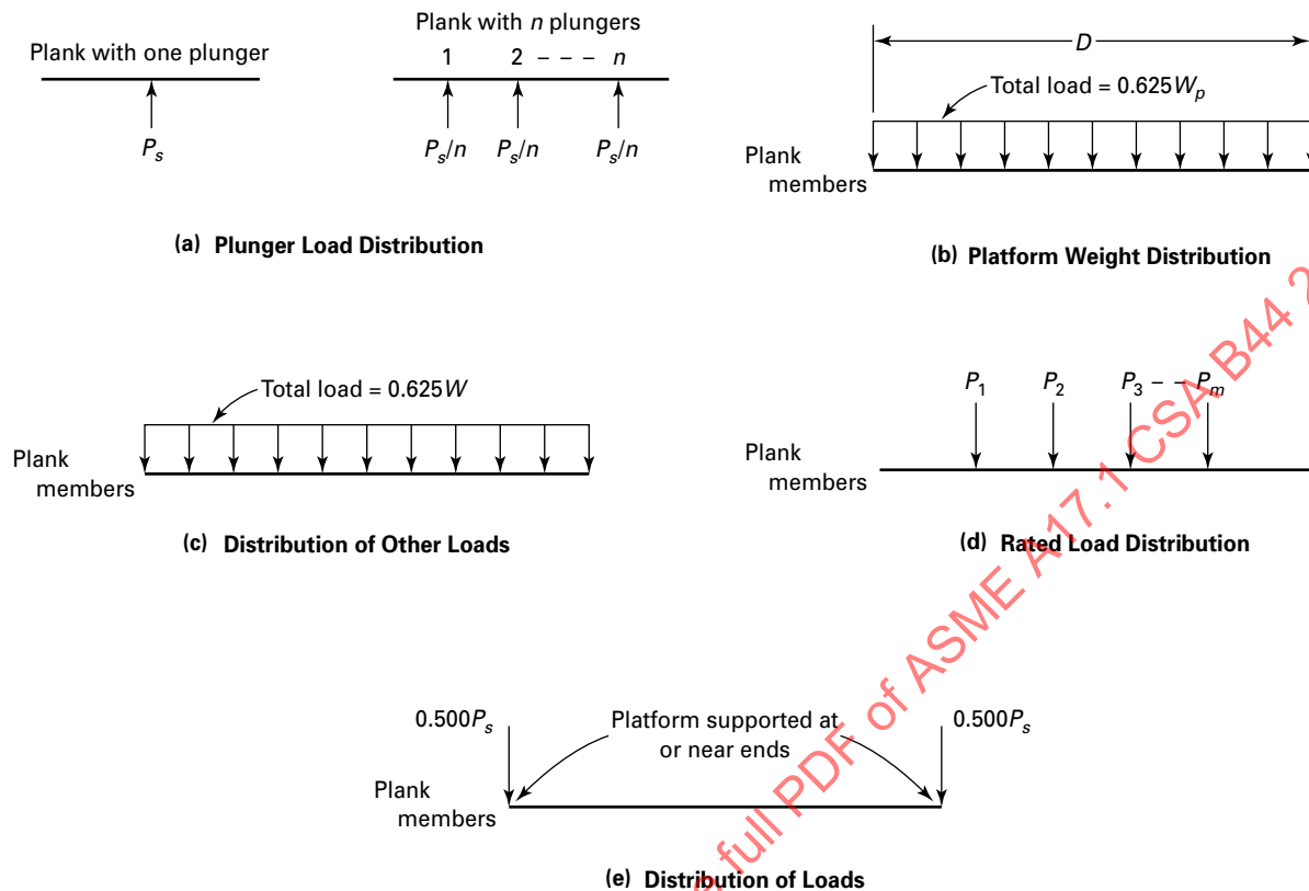
Figure 8.2.9.1.3 Load Distribution
