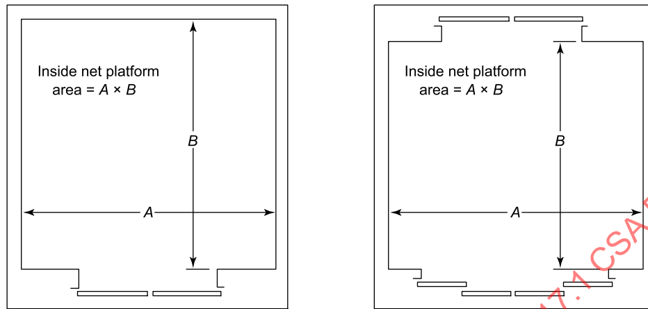
Figure 2.16.1.1 Inside Net Platform Areas for Passenger Elevators
