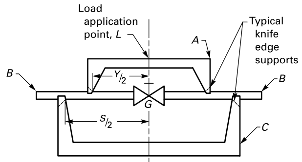
Figure 4.4.4-1 Test Assembly
