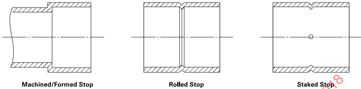
Figure 8-1 Tube Stops
