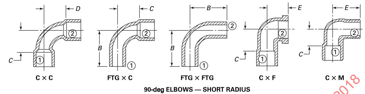
Figure 4.1-1 Method of Designating Laying Lengths of Fittings and Openings of Reducing Fittings (Cont'd)
