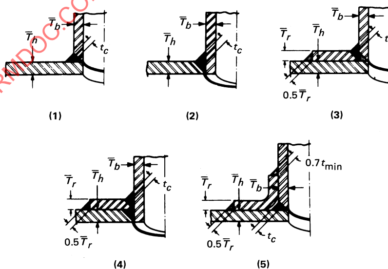
Fig. 328.5.4D Acceptable Details for Branch Attachment Welds
