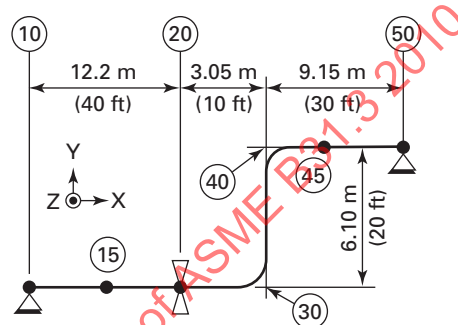
Fig. S301.1 Simple Code Compliant Model
