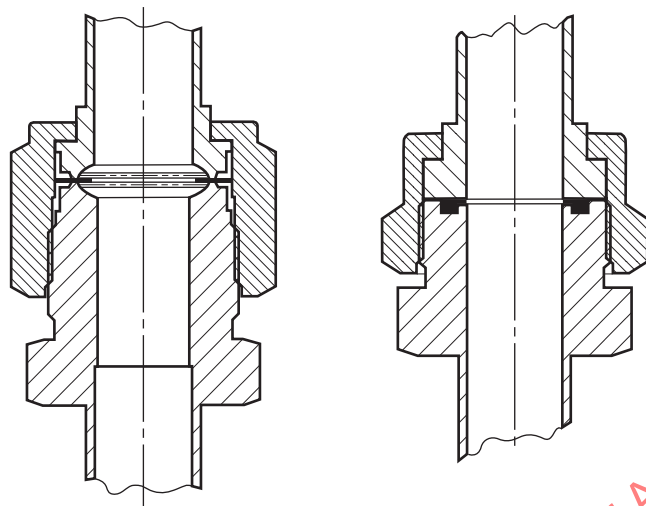
Fig. U335.7.1 Face Seal Joints
