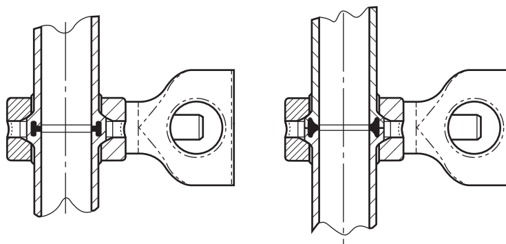
Fig. U335.8 Hygienic Clamp
