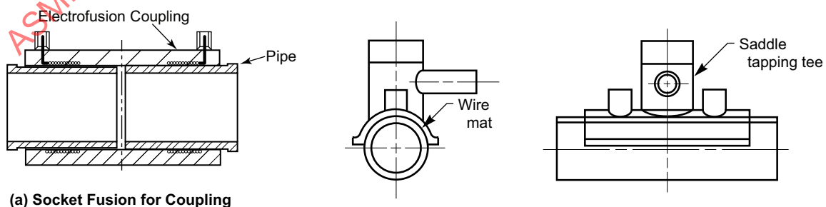
(a) Socket Fusion for Coupling
