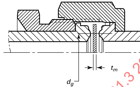
(b) Metal Face Seal
