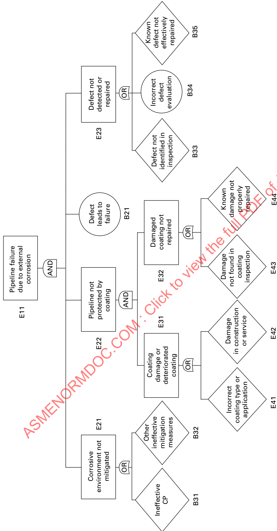
Figure 5.4-1 Fault Tree for External Corrosion
