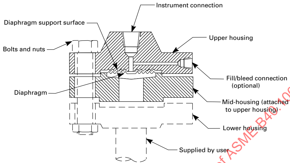
Figure 3-1.2.2.4-2 Upper Housing, Removable
