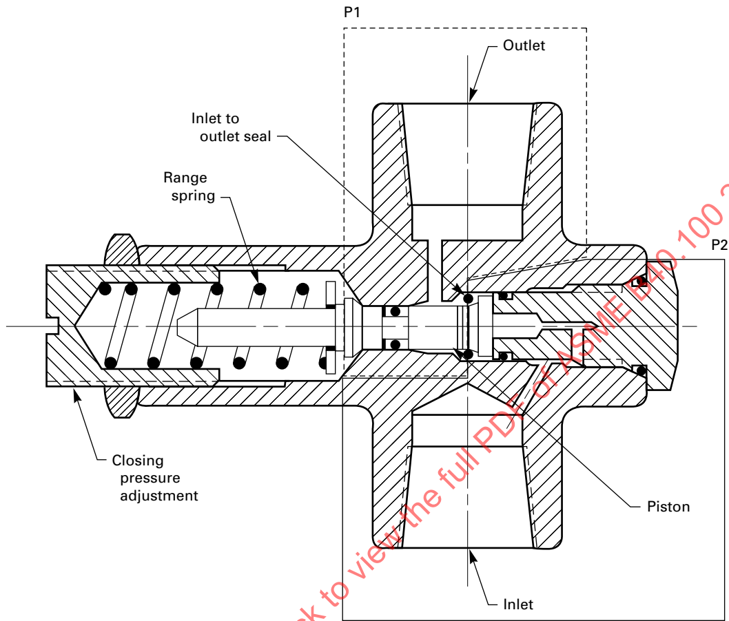
Figure 5-2.1-1 Piston Type
