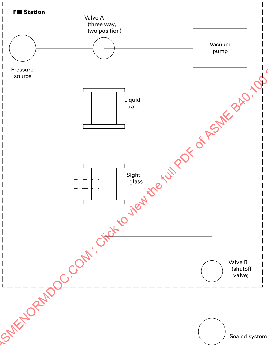
Figure 3-1.8.2-1 Sealed Setting
