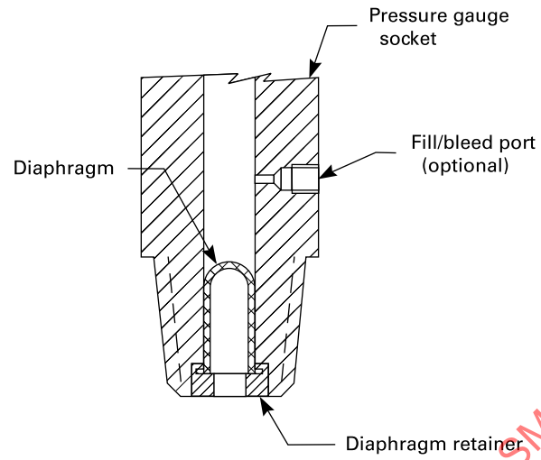
Figure 3-1.2.14-1 Gauge Isolator
