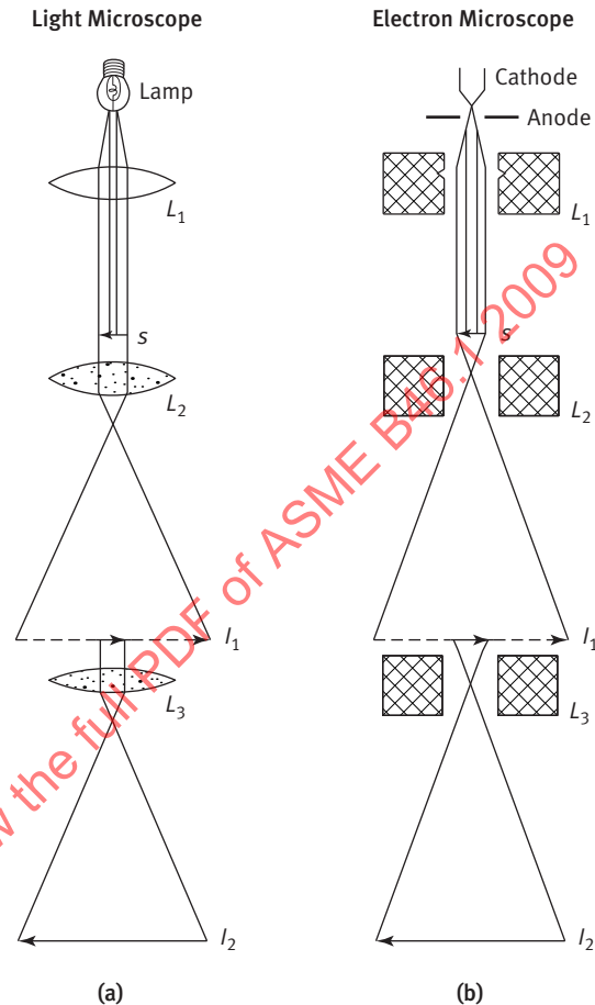
Fig. C-8 Comparison of Optical and Transmission Electron Microscope
