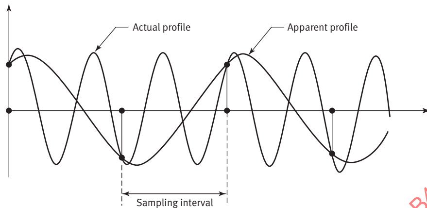
Fig. 3-4 Aliasing
