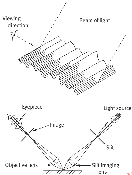
Fig. C-1 Schmaltz Profile Microscope
