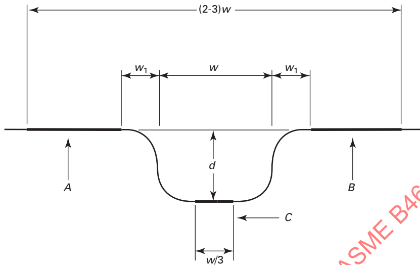
Fig. 11-4 Assessment of Calibrated Values for Type A1
