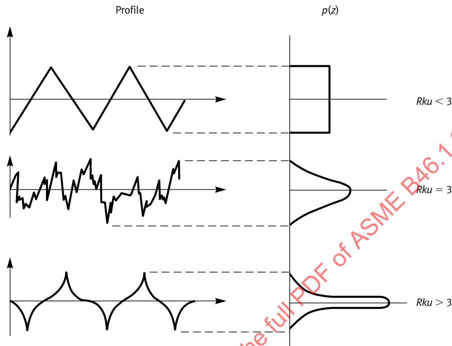
Fig. 1-19 Three Surface Profiles With Different Kurtosis
