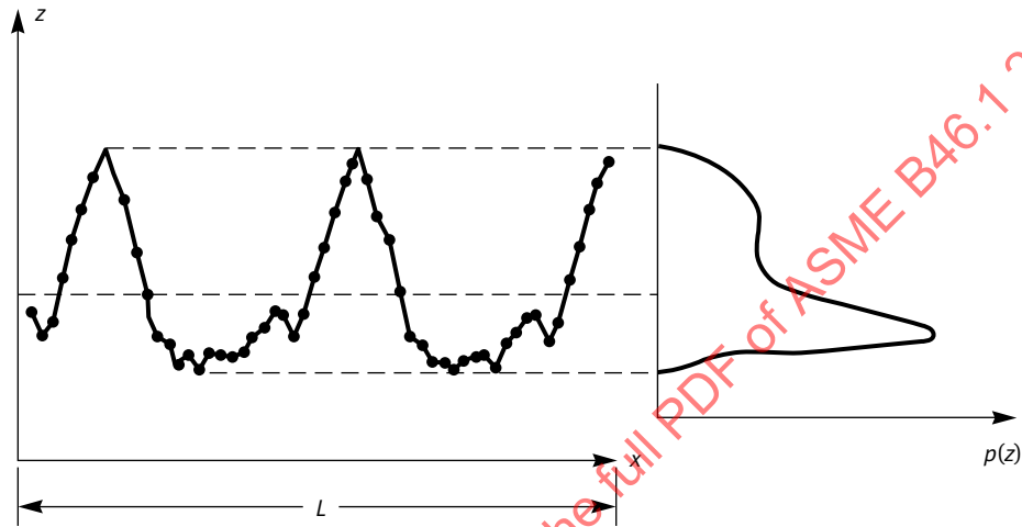
Fig. 1-15 Amplitude Density Function — ADF(z) or p(z)
