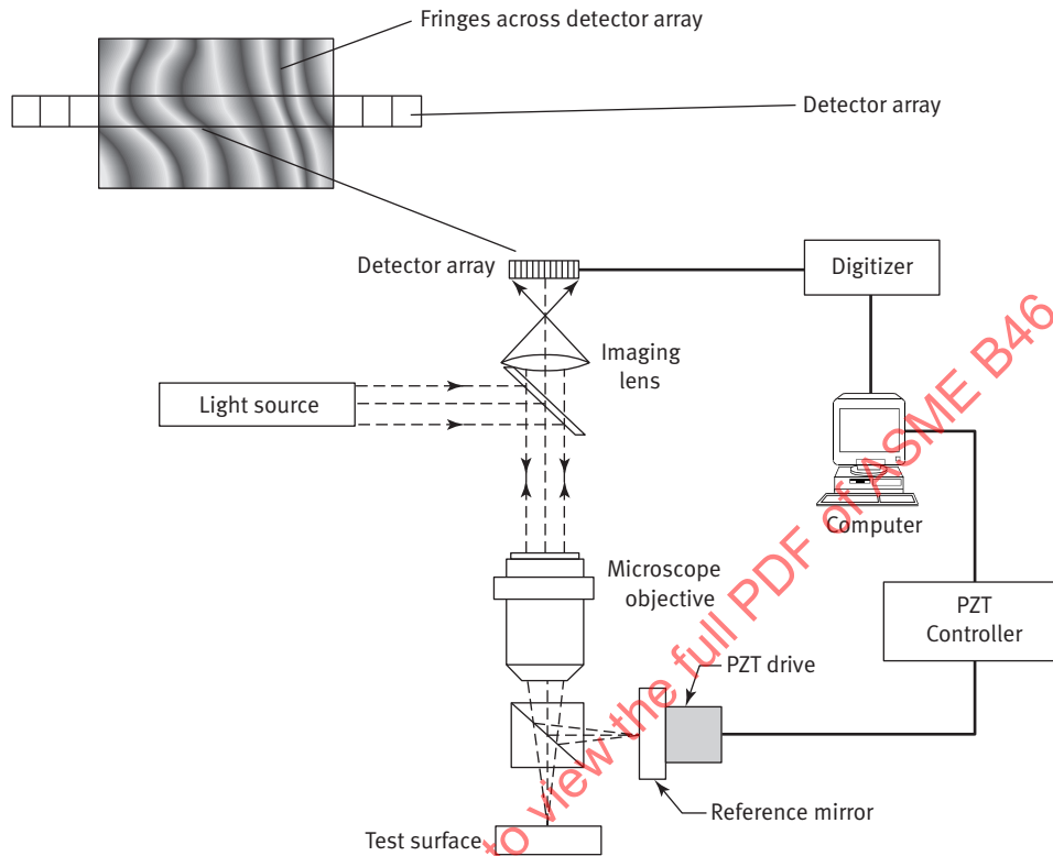
Fig. 8-1 A Typical Phase Measuring Interferometer System
