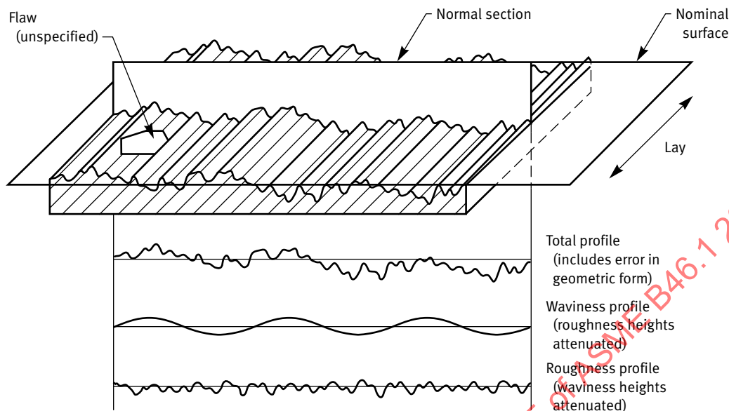
Fig. 1-1 Schematic Diagram of Surface Characteristics
