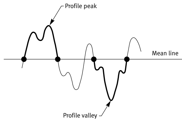
Fig. 1-6 Profile Peak and Valley
