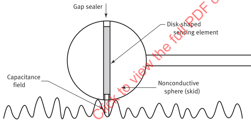
(b) Typical Fringe-Field Capacitance Probe
