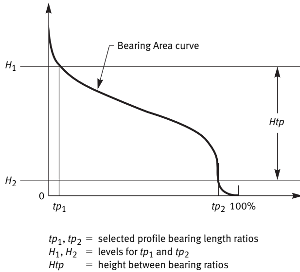
Fig. 1-17 The Bearing Area Curve and Related Parameters
