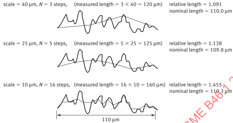
Fig. 10-4 Three Stepping Exercises From a Length-Scale Analysis on a Simulated Profile
