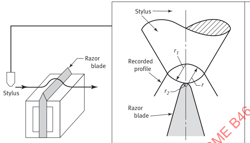
Fig. 11-7 Use of Type B3 Specimen
