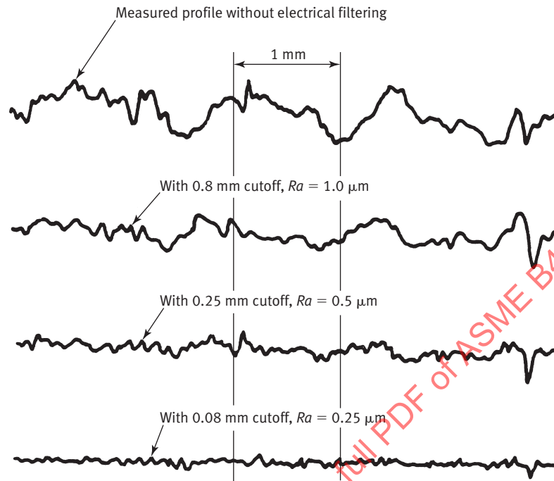
Fig. 4-2 Effects of Various Cutoff Values
