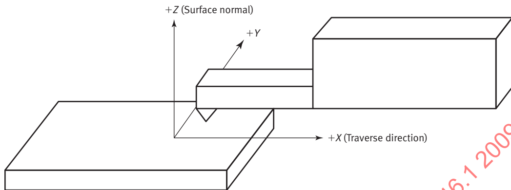
Fig. 3-1 Profile Coordinate System
