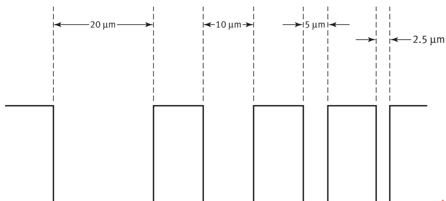
Fig. 11-5 Type B1 Grooves: Set of Four Grooves
