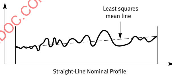
Fig. 1-4 Examples of Nominal Profiles
