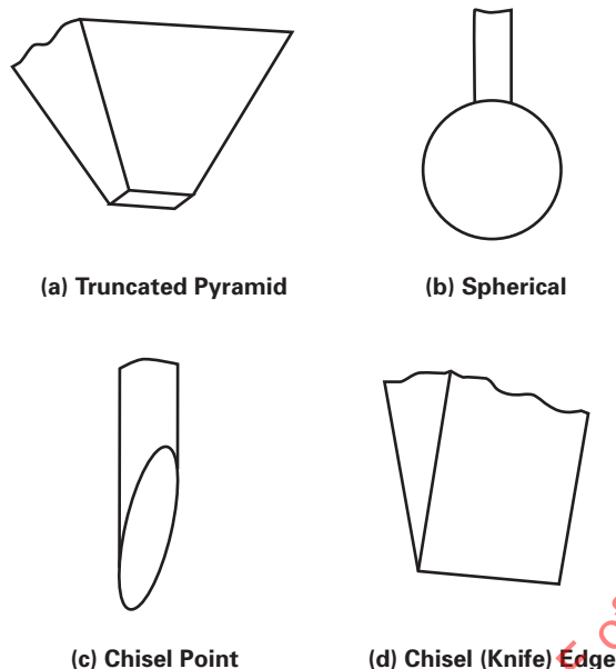
Fig. 3-3 Other Stylus Tip Geometries
