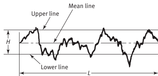
Fig. D-3 Swedish Height of Irregularities
