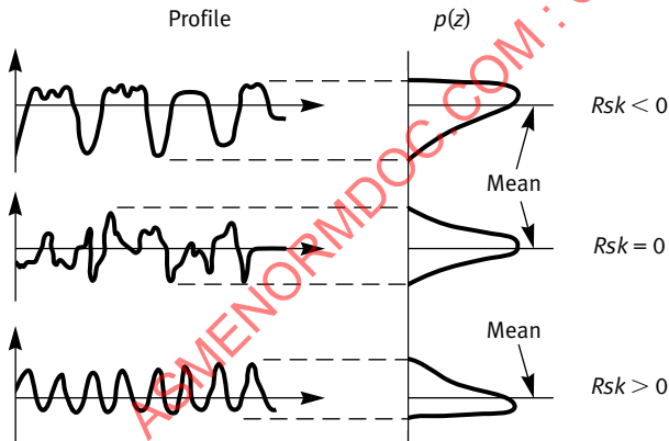
Fig. 1-18 Three Surface Profiles With Different Skewness
