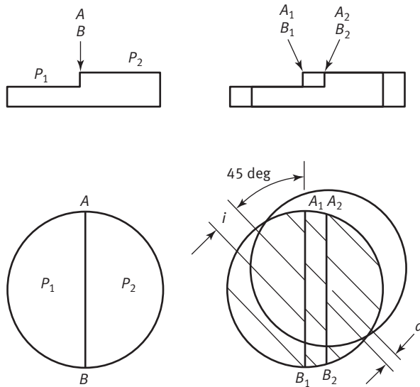
Fig. C-6 Differential Interferometry
