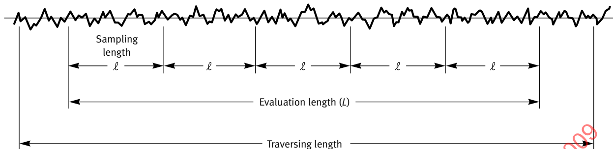
Fig. 1-7 Surface Profile Measurement Lengths
