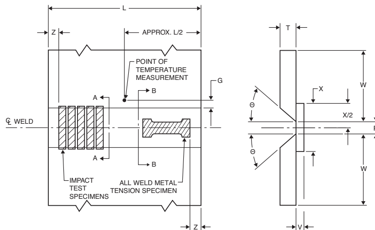
(A) JOINT CONFIGURATION AND LOCATION OF TEST SPECIMENS
