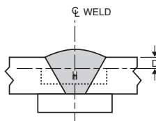
(A) JOINT CONFIGURATION AND LOCATION OF TEST SPECIMENS
