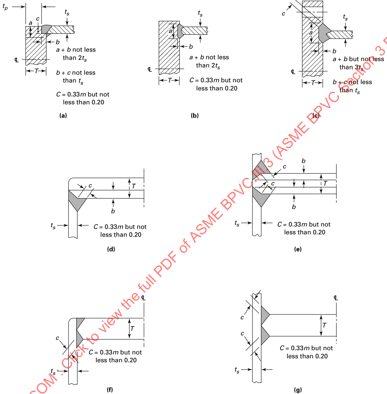
Figure WC-3225-3 Attachment of Flat Heads to Containment Shell
