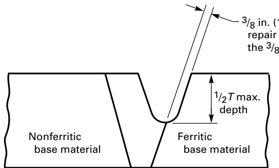
Figure WB-4622.11(c)(6)-1 Temper Bead Weld Repair and Weld Temper Bead Reinforcement of Dissimilar Metal Welds or Buttering
