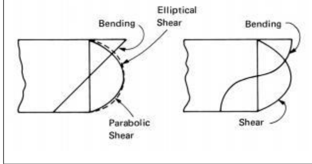
Figure A-9531-1 Bending and Shear Stresses
