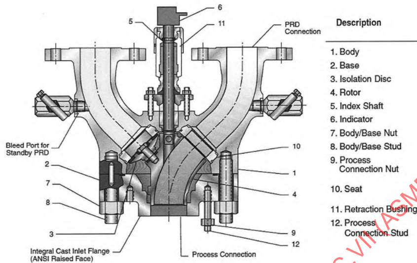
Figure 103.1.4-1 Changeover Valve
