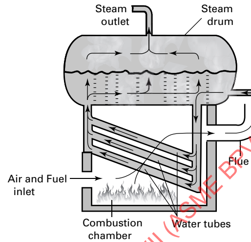
Horizontal Tubes
