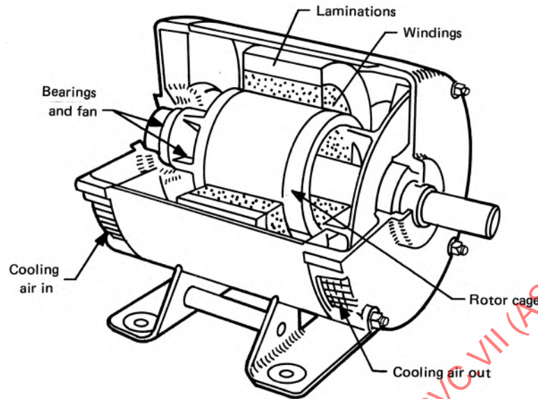
Figure 102.5-1 Typical Motor Drive
