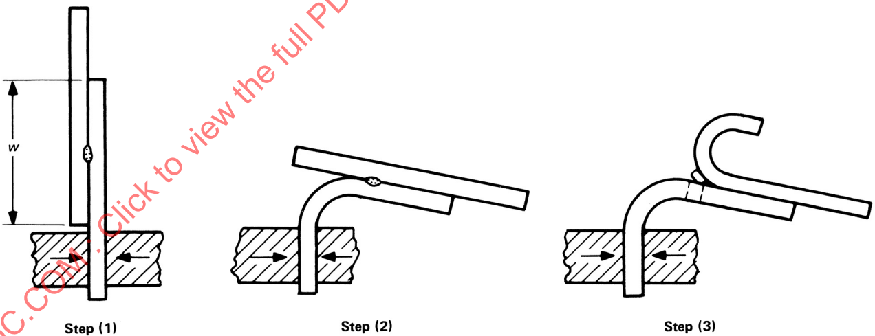
Figure 17-16 Peel Test
