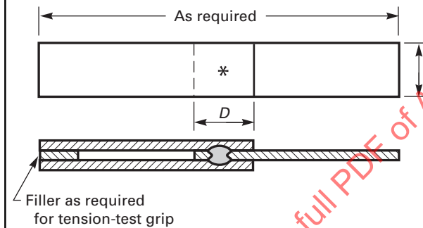
Figure 17-9 Single Spot-Weld Tension Specimen for Three-Ply Joint
