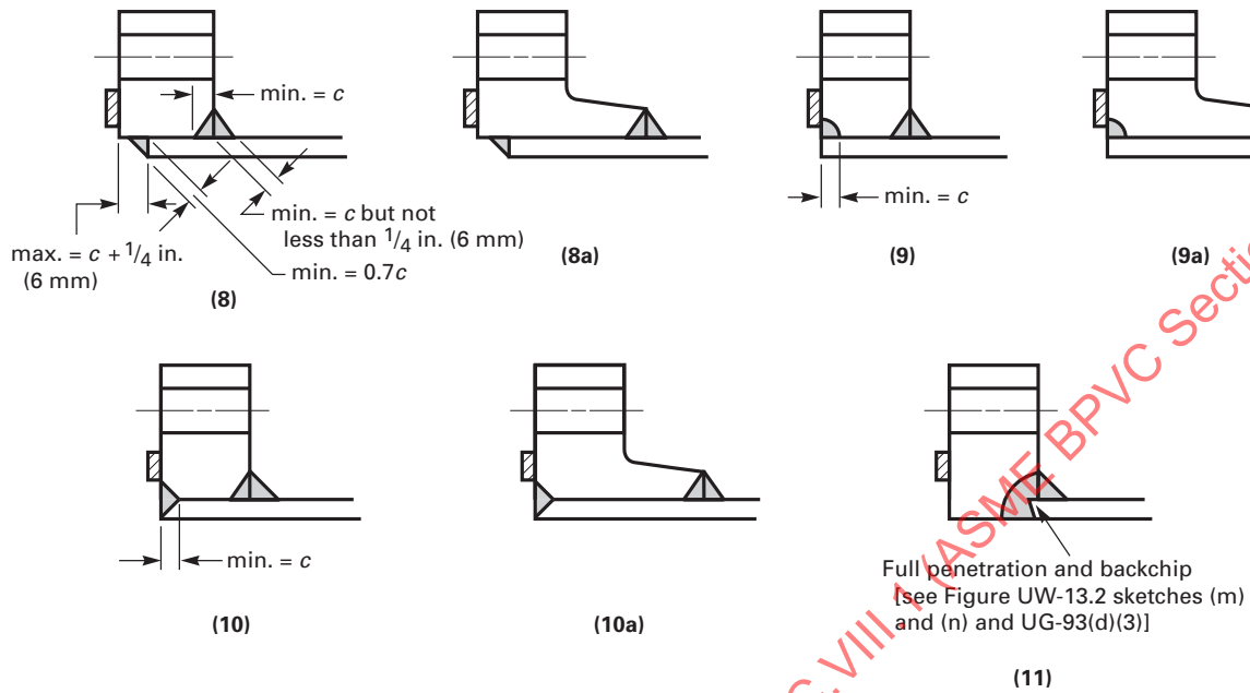
Figure 2-4 Types of Flanges (Cont'd)
