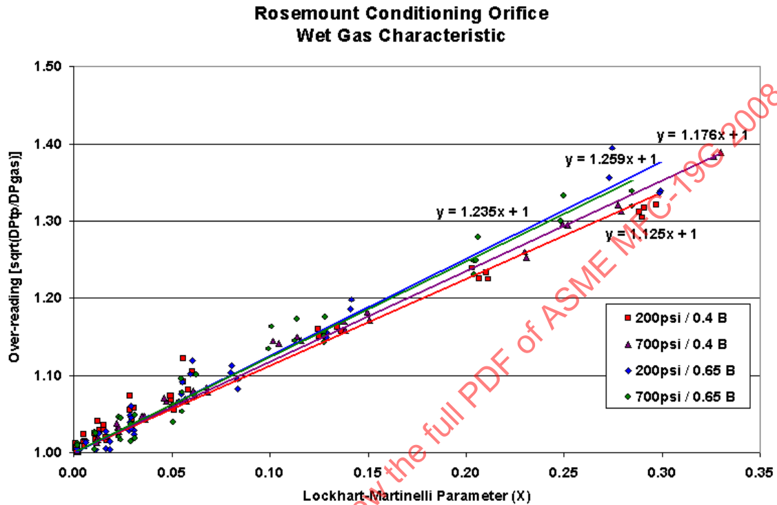
Fig. G-8 The Four-Hole Orifice Plate Meter Wet Gas Flow Results
