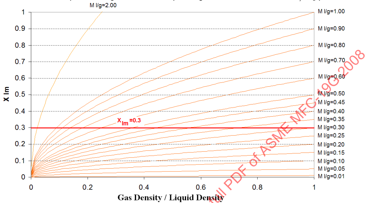
Fig. D-4 Constant Liquid Mass Flow Rate to Gas Mass Flow Rate Ratio Lines Plotted on Gas-to-Liquid Density Ratio to the Lockhart–Martinelli Parameter
