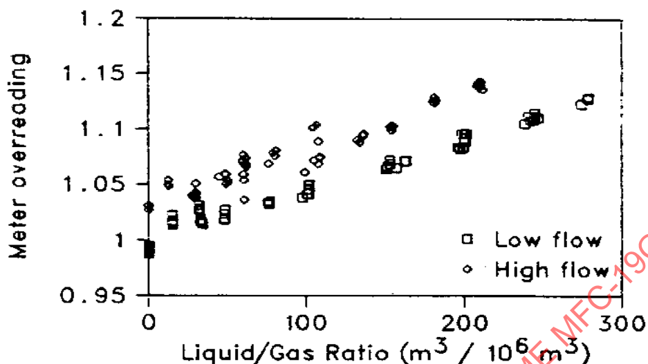
Fig. 6.1.2.2-1 Washington [25, 26] Field Data for Wet Natural Gas Flow
