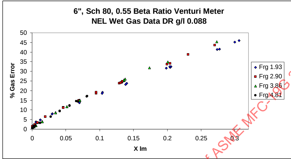
Fig. G-1 NEL / DTI 6 in., 0.55 Beta Venturi Meter Wet Gas Data Set With Fixed Pressure / Gas-to-Liquid Density Ratios (DR g/l), and Separate Gas Densimetric Froude Numbers
