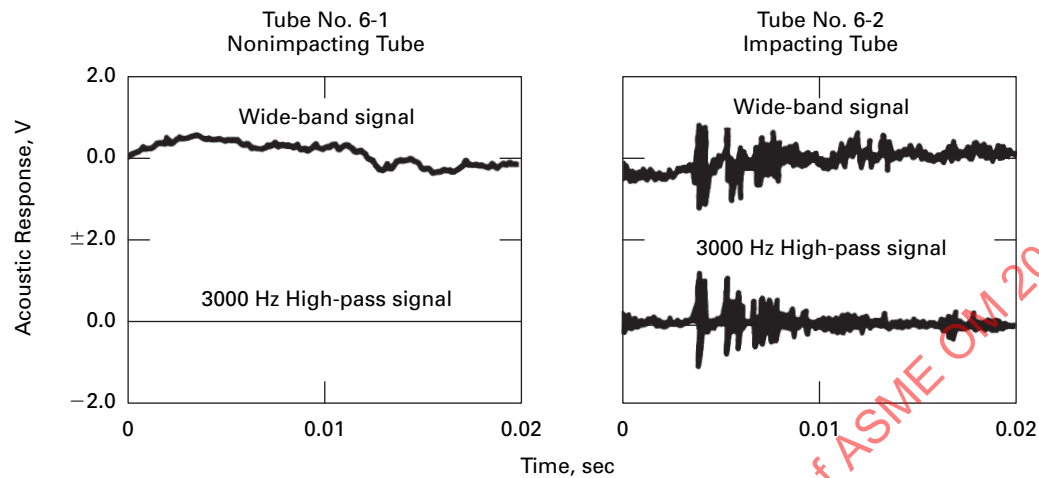
(a) Time History Plots for Impacting and Nonimpacting Tubes
