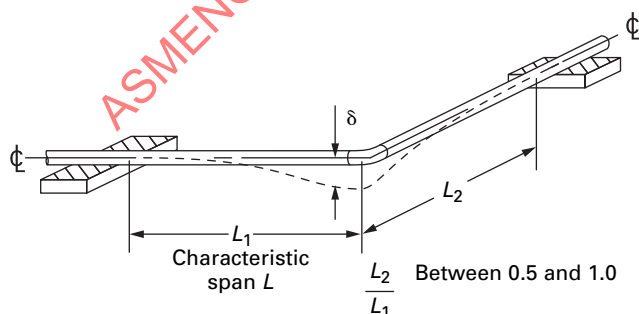
Fig. 8 Span/Elbow Span Out-of-Plane Deflection Measurement, Span Ratio > 0.5
