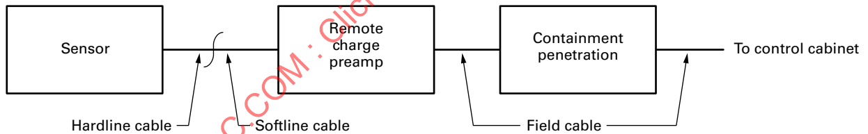
Fig. 4 Field Equipment
