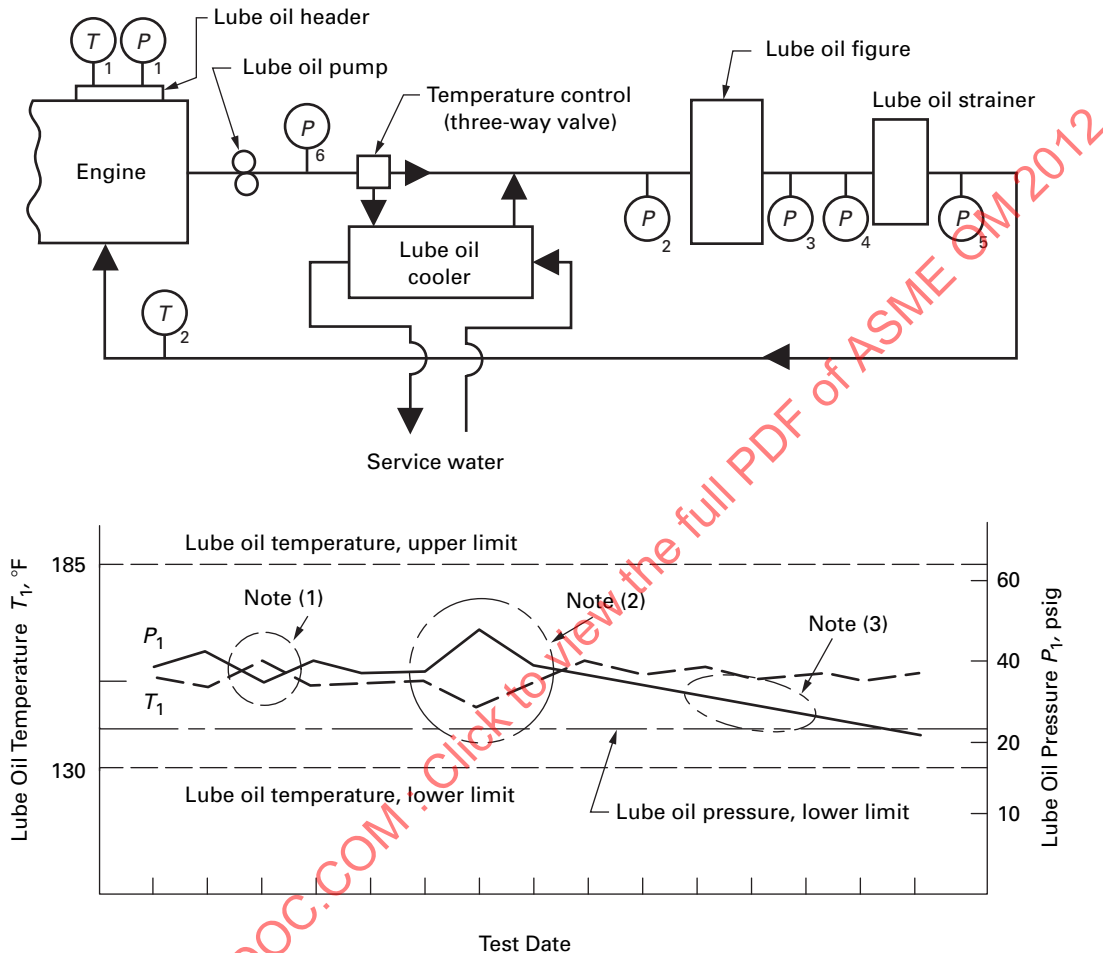
Trend Plotting — Lube Oil Temperature T_1 and Lube Oil Pressure P_1
