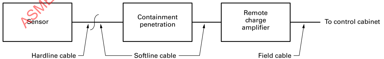
(b) For Remote Charge Amplifier Outside Containment
