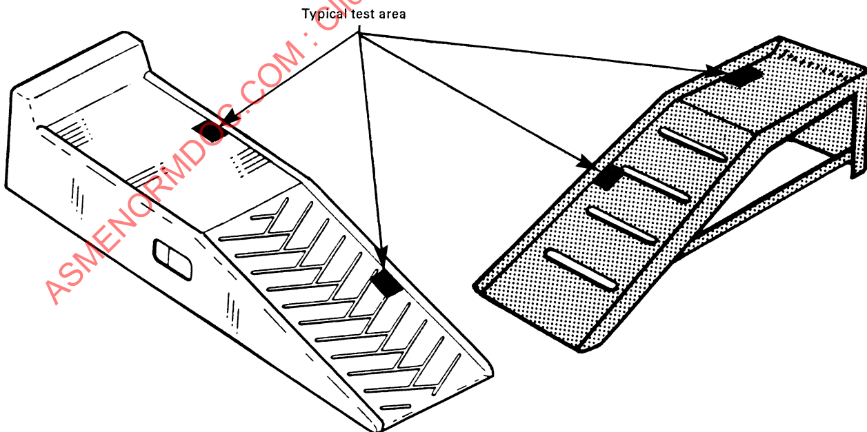
Fig. 14-4.1.1-1 Typical Test Area for Off-Center Load Test
