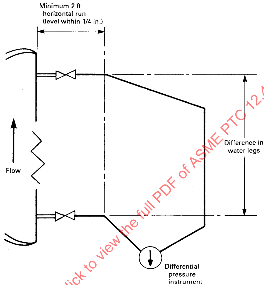
FIG. 4.1 WATER LEG DETERMINATION
