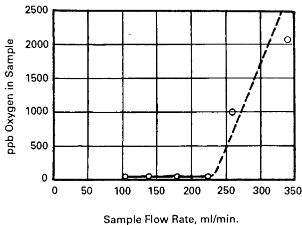
FIG. 4.5 OXYGEN CONTENT OF SAMPLE
