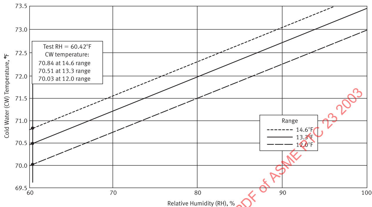
Fig. F2-2 Cross Plot No. 1B Dry Bulb = 56.12°F, Water Flow Rate = 378,000 gpm (100%)
