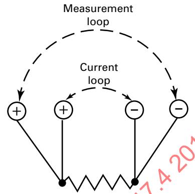
(a) Four-Wire RTD
