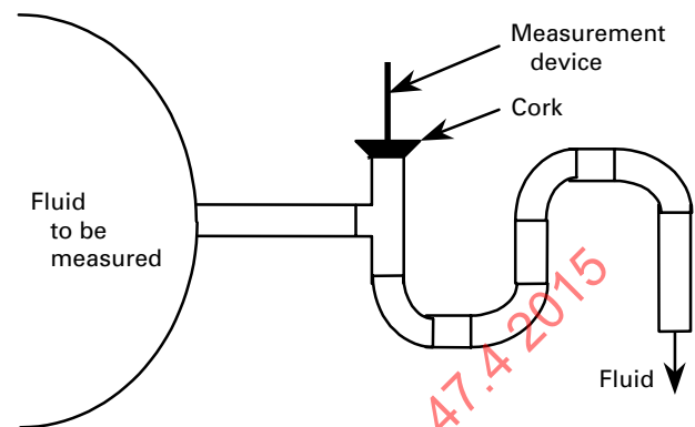
Fig. 4-3.6.2-1 Flow-Through Well
