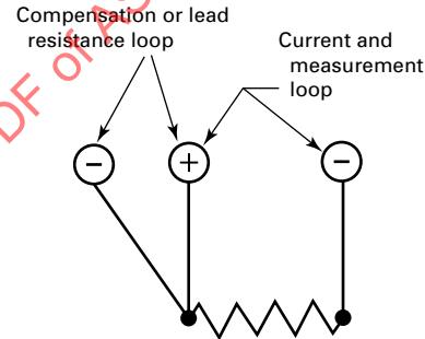
(b) Three-Wire RTD
