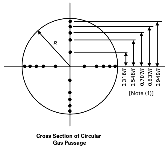
Fig. 4-3.6.3-1 Duct Measurement Points
