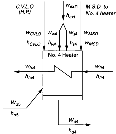
FIG. 9.6 NO. 4 HEATER EXTRACTION FLOW AND ENTHALPY
