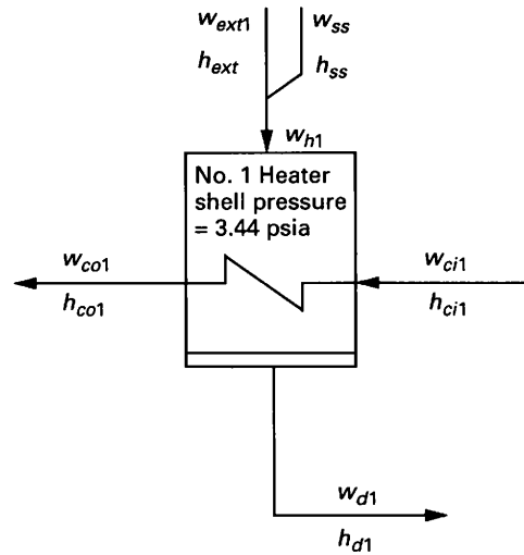
FIG. 9.9 NO. 1 HEATER EXTRACTION FLOW
