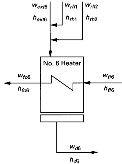
FIG. 9.4 NO. 6 HEATER EXTRACTION FLOW AND ENTHALPY
