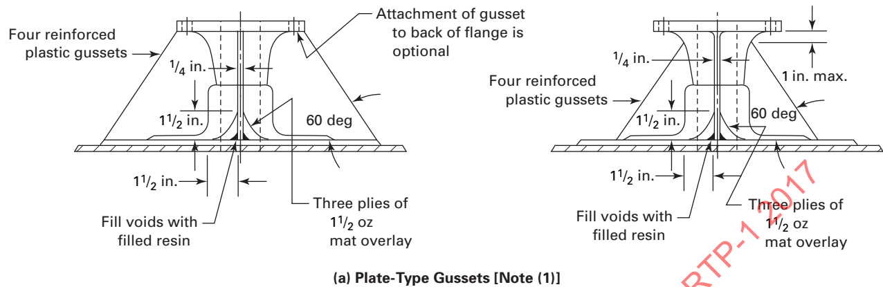
Fig. 4-13 Nozzle Gussets
