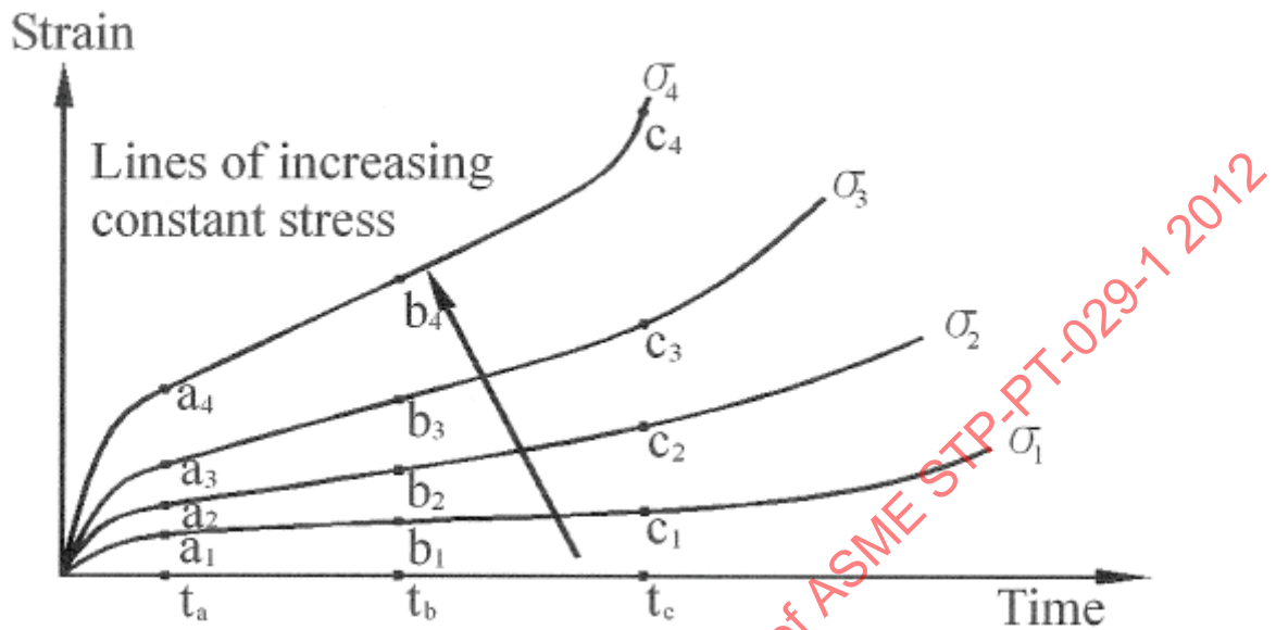
Figure 1 - Creep Curves Conventionally Plotted as Strain vs Time at Constant Stress.
