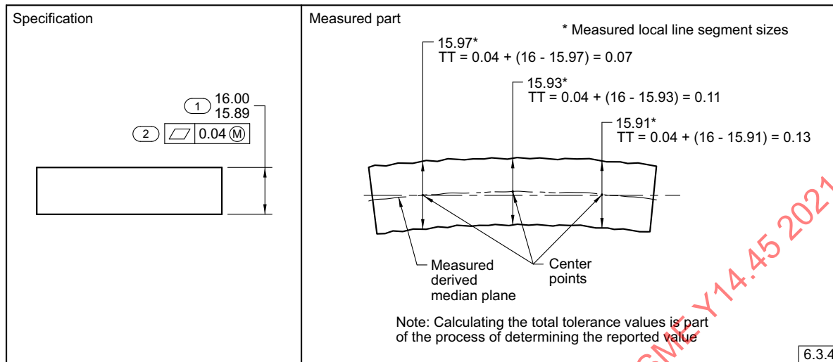
Figure 6-17 Flatness at MMC, Resolved Geometry Method
