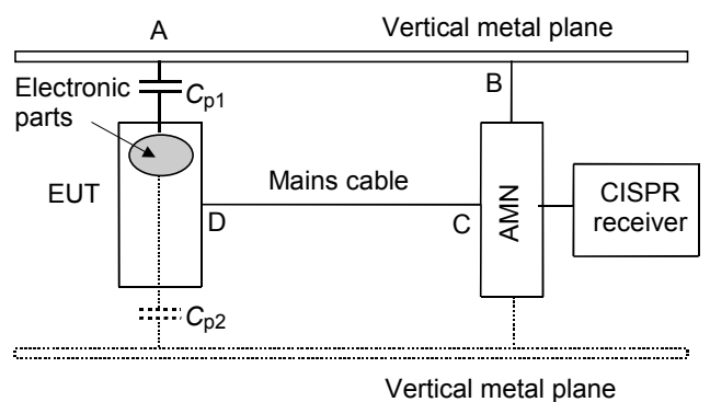
Figure 16 – Variation of the parasitic capacitance, and hence of the CM-impedance, by changing the position of the reference plane (non-conducting EUT housing)
