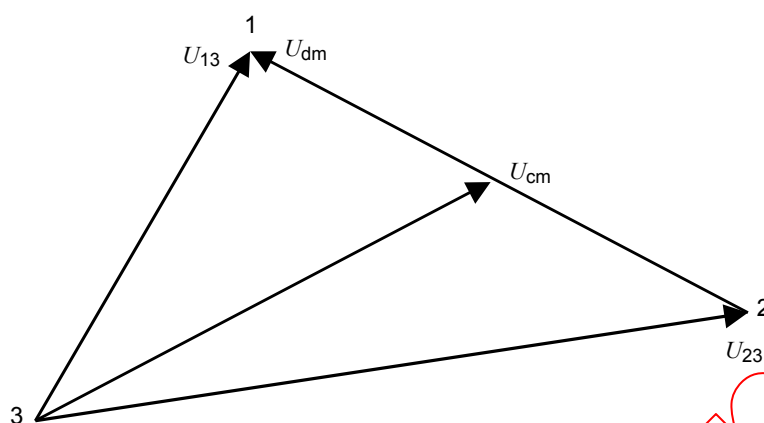
Figure 12 – Relation between the voltages
