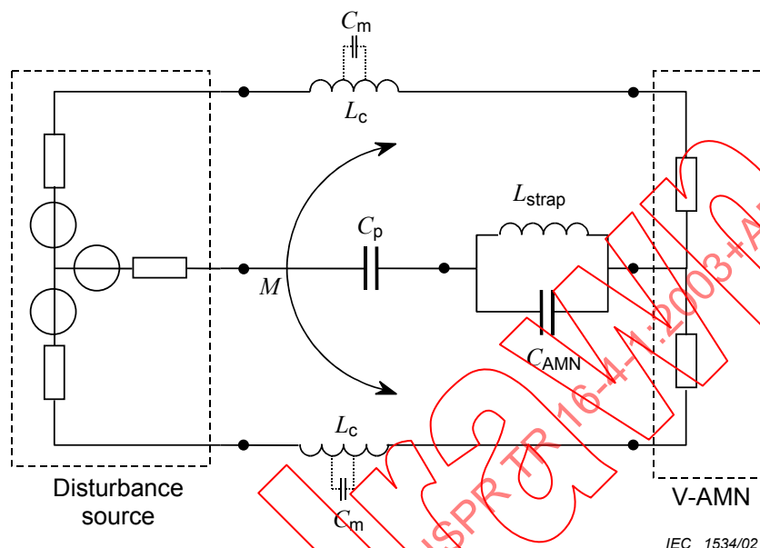
Figure 17 – Influence quantities in between the EUT (disturbance source) and the V-AMN
