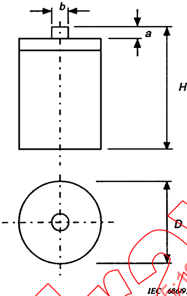
Figure 4 – Jacketed cylindrical cells interchangeable with primary batteries
