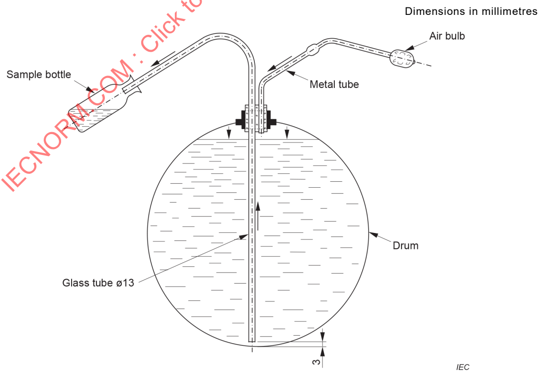
Figure 4 – Siphon
