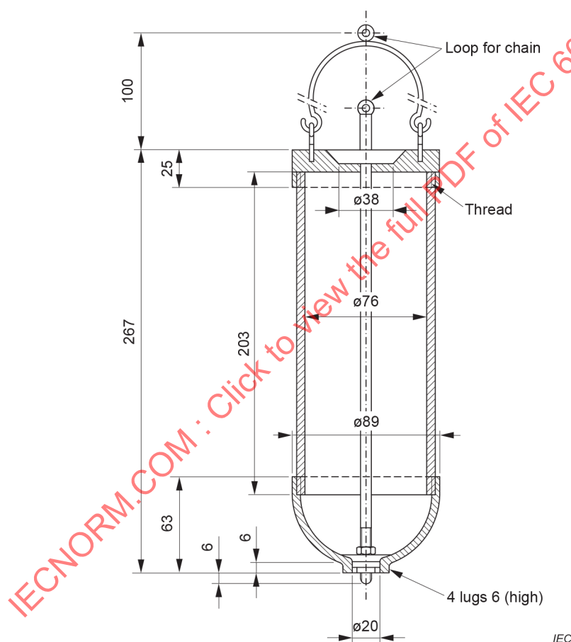
Figure 1 – Thief dipper
