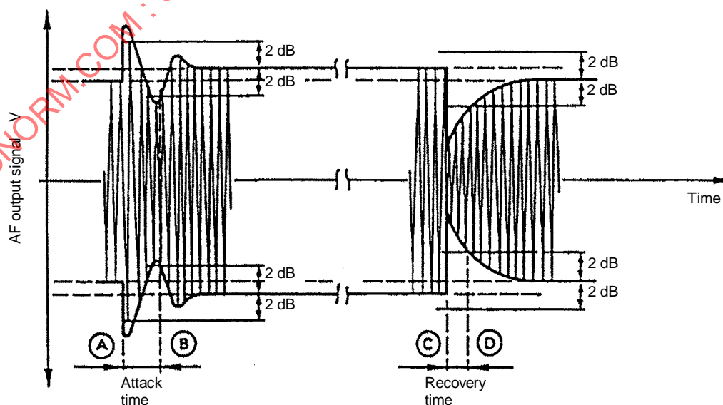
Figure 7 – Example of dynamic AGC characteristic
