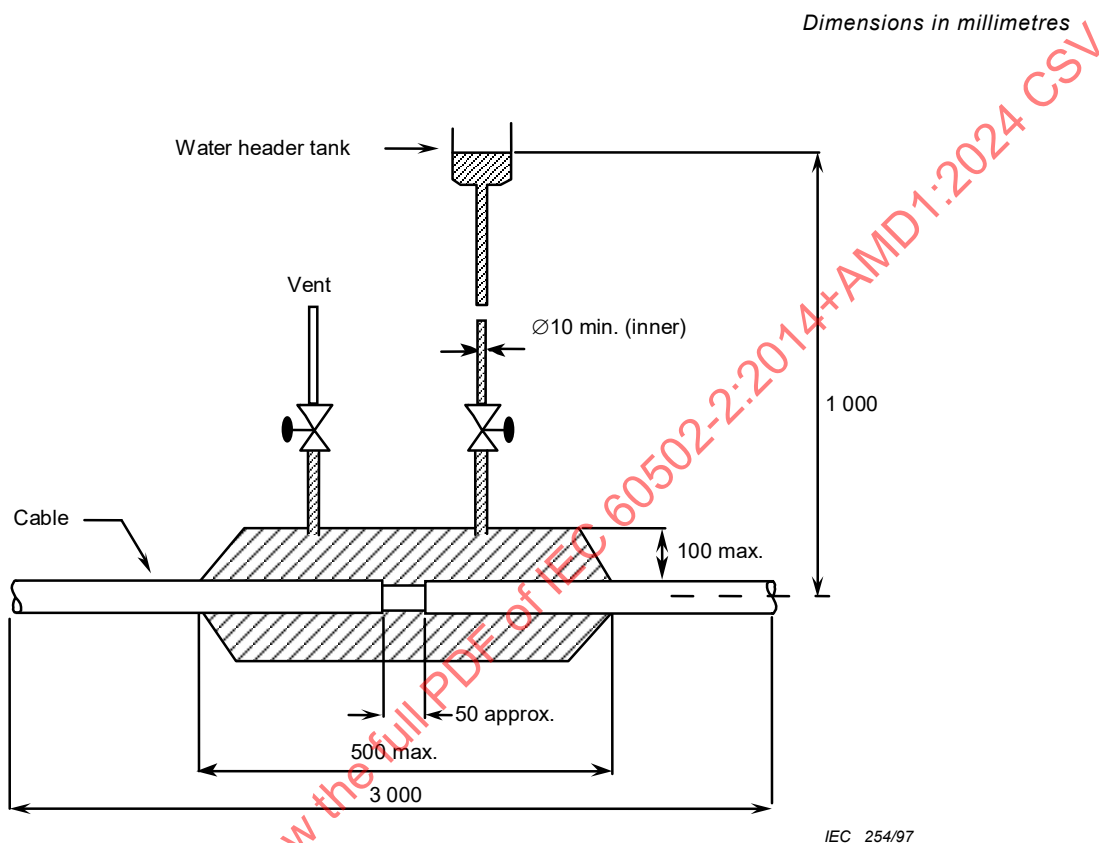
Figure F.1 – Schematic diagram of apparatus for water penetration test
