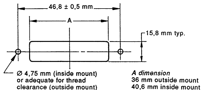
Figure 18 – Connector panel cut-out
