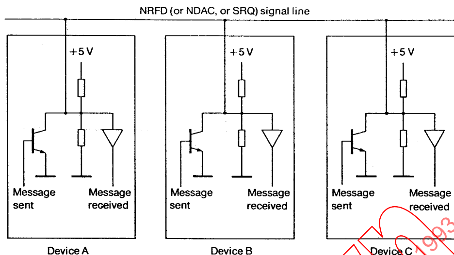
Figure 23 – Bi-state signal line logic (open collector drivers)
