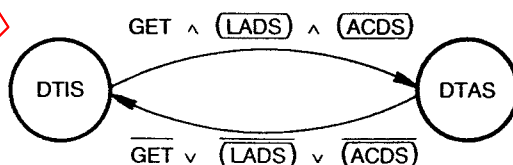
Figure 13 – Device trigger state diagram
