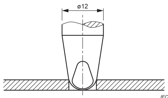
Figure 103 – Demonstration of the non-penetration of the internal volume
