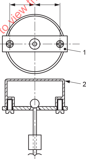
Figure 113 – Example of mounting block for boxes to be embedded in masonry (flush type and semi-flush type)
