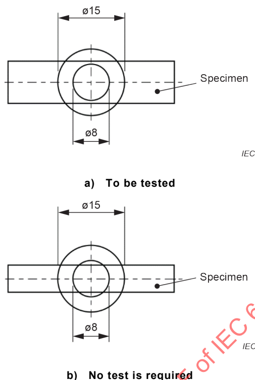
Figure 130 – Diagrammatic representation of the glow-wire test
