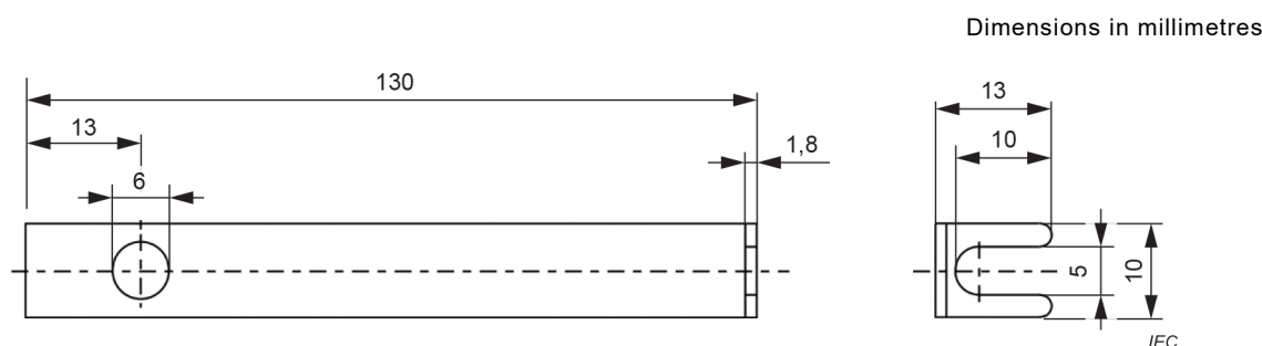
Figure 105 – Test strap
