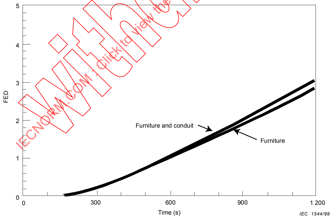
Figure B.8 – Relative increase of toxicity due to exposed conduit (concrete wall)
