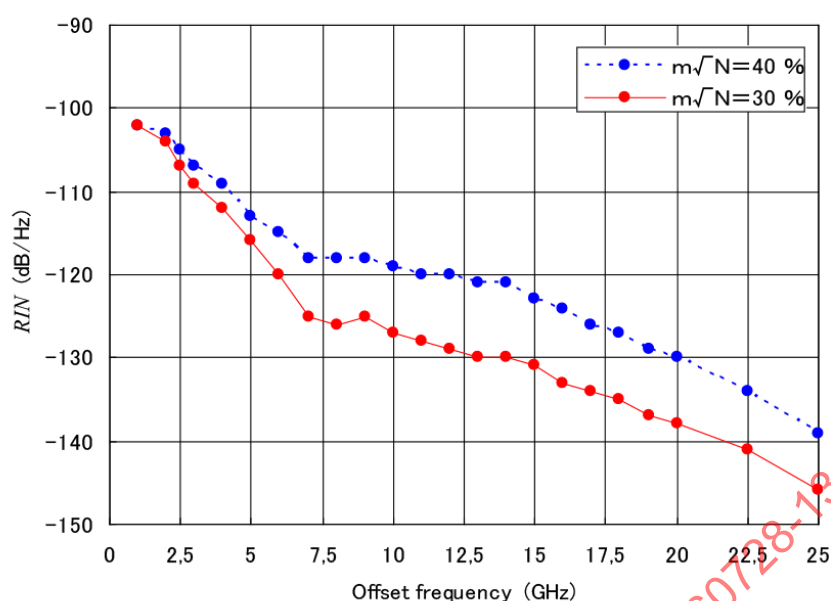
Figure C.1 – Experimental results of R/N degradation due to optical beat
