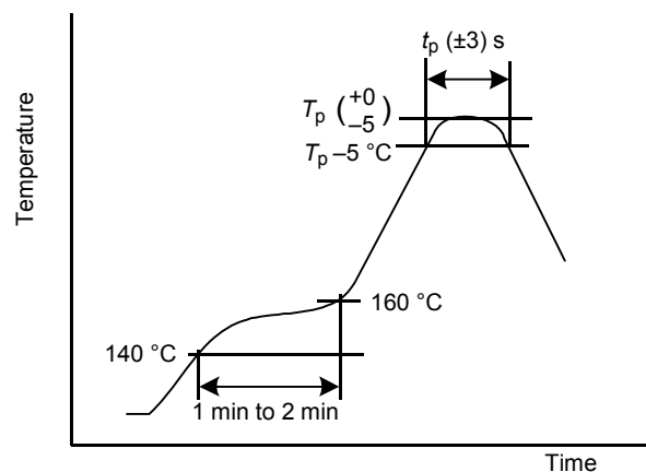
Figure A.9 – Temperature profile of infrared convection and convection reflow soldering for Sn-Pb eutectic assembly
