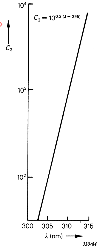
Figure 3 – Correction factor C_2 for \lambda = 302,5 nm to 315 nm
