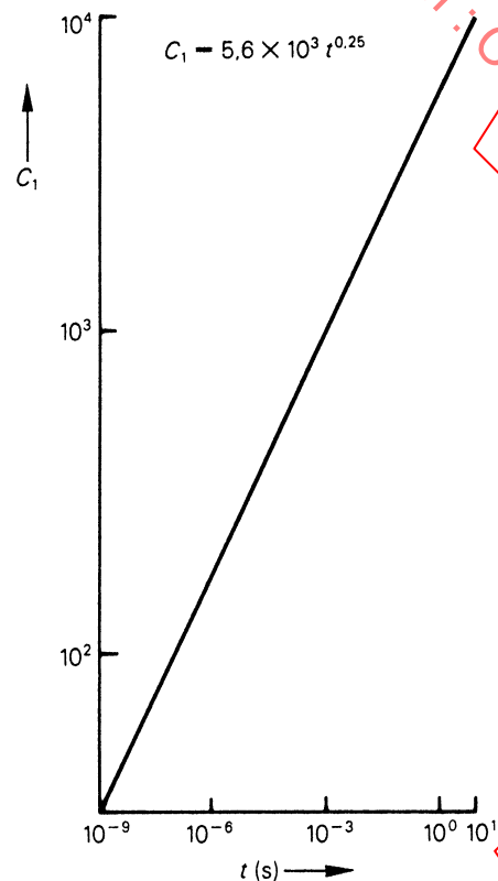
Figure 1 – Correction factor C_1 for emission durations from 10^{-9} s to 10 s
