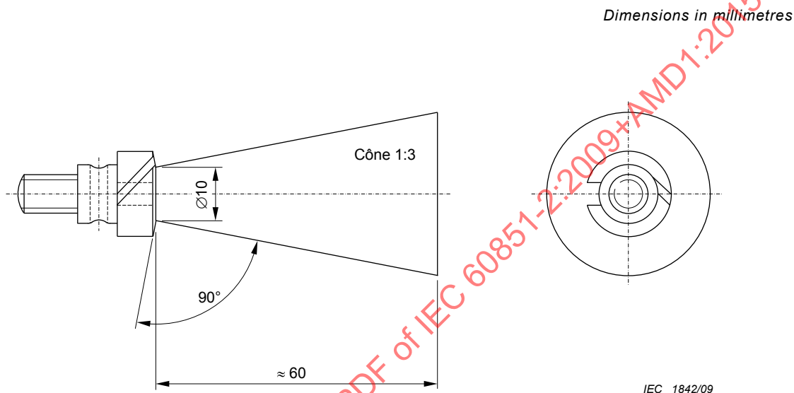
Figure 1 – Conical mandrel
