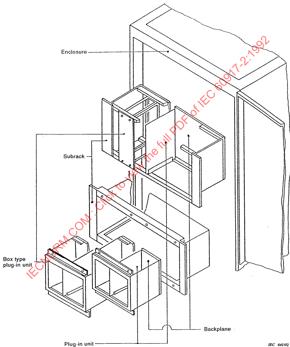
Figure 2 – Arrangement of plug-in units, subracks and enclosures
