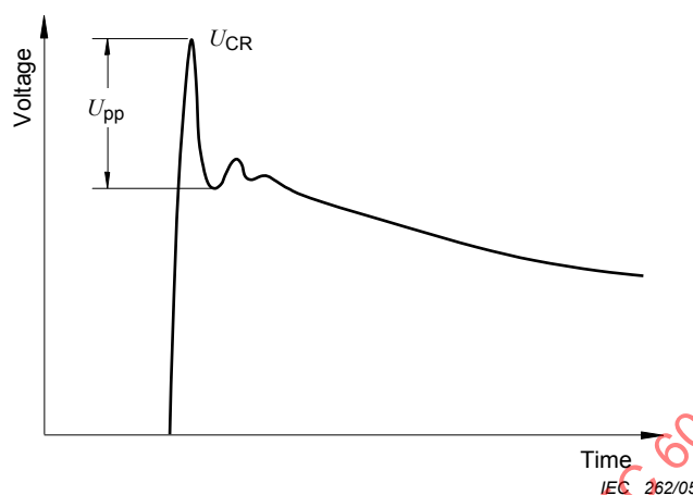
Figure 1 – Impulse wave form
