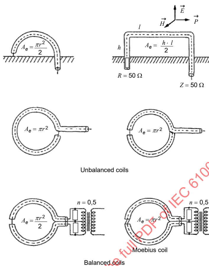
Figure C.1 – Magnetic field sensors [23]
