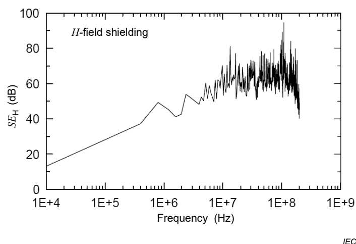
Figure 3 – Measured magnetic field shielding effectiveness SE_H for a building
