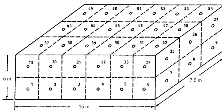
Figure 32 – Example of antenna locations for the localized antenna tests for a hypothetical shielded enclosure or facility
