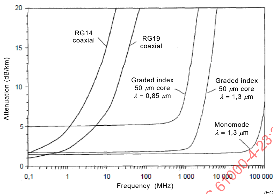
Figure C.12 – Attenuation of coaxial lines and fibre optic cables as a function of frequency
