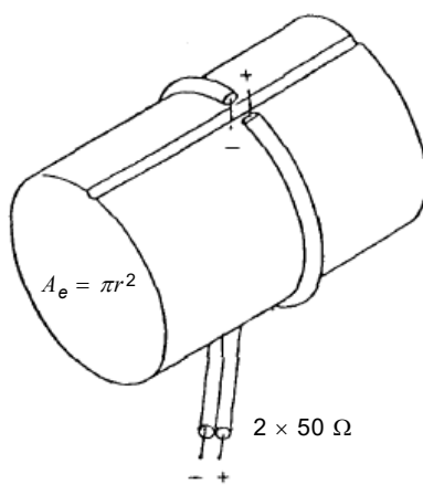
Figure C.2 – Single-slot, cylindrical coil sensor [23]
