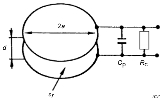
Figure C.4 – Electrical configuration of an E -field sensor [23]
