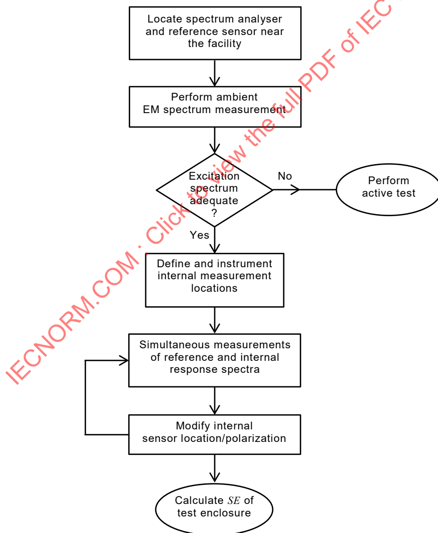
Figure 26 – Test procedure for the ambient EM excitation test
