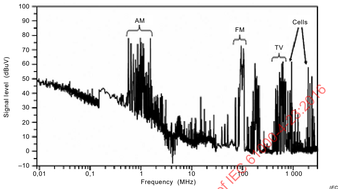
Figure 25 – Example scan from 9 kHz to 3 GHz for the ambient electromagnetic field from communication signals
