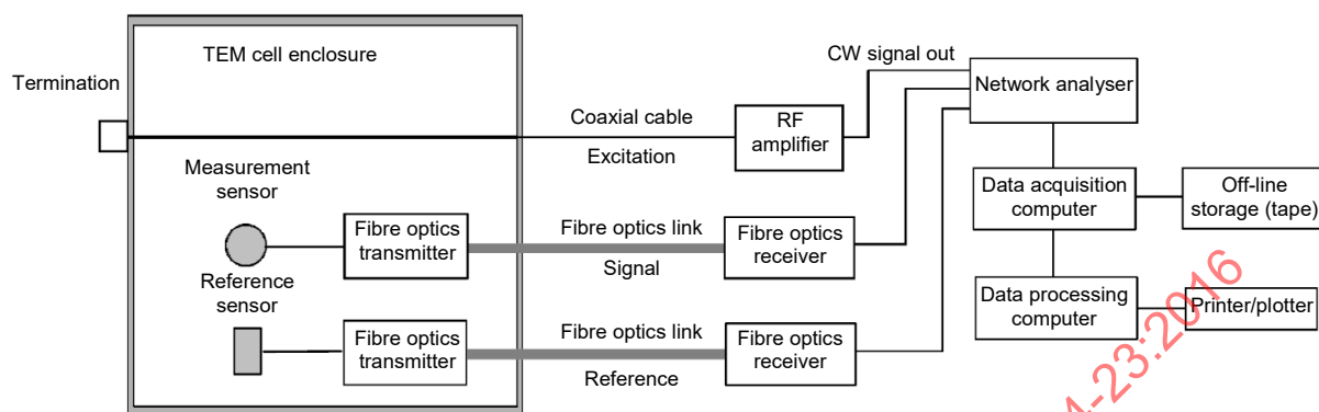
Figure 28 – Example test set-up for field illumination in the TEM cell
