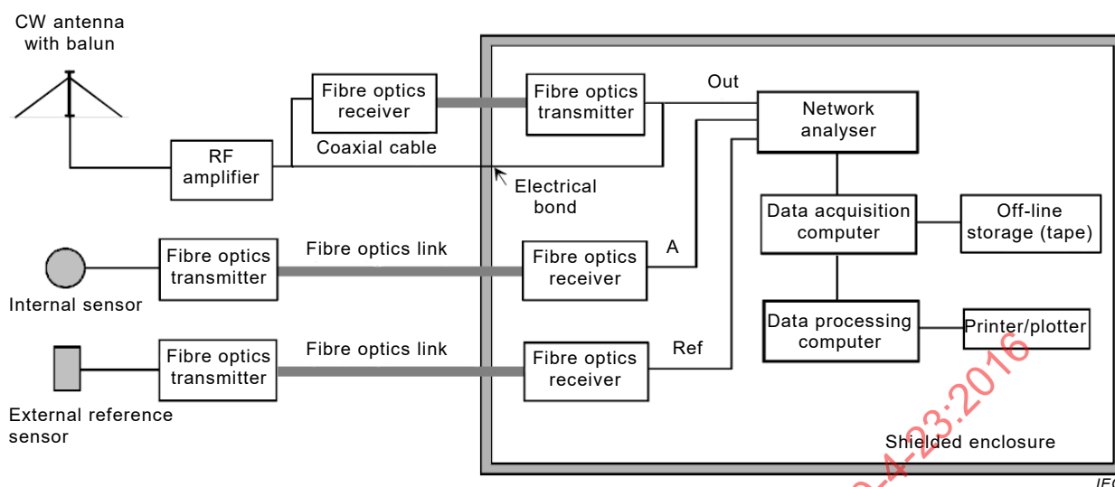
Figure 22 – Example CW measurement set-up
