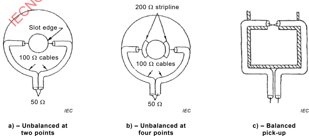
Figure C.10 – Voltage pick-up points on the edges of the toroidal sensor [23]
