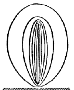
Figure C.7 – Equipotential shapes for an optimally designed E -field sensor [23]
