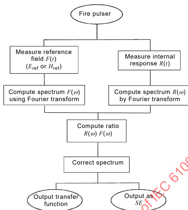
Figure 20 – Test procedure for the pulse test
