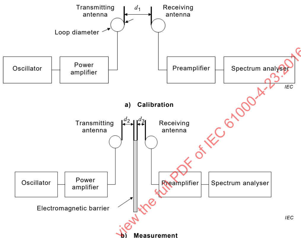
Figure 31 – Test set-up for the H -field shielding effectiveness measurements
