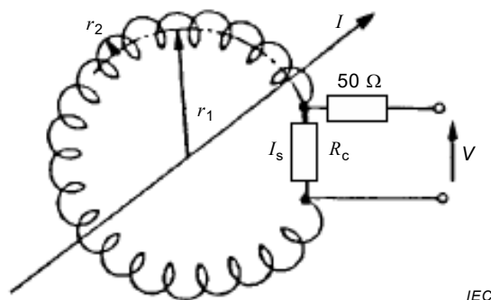
Figure C.8 – Rogowski coil used for current measurements [23]
