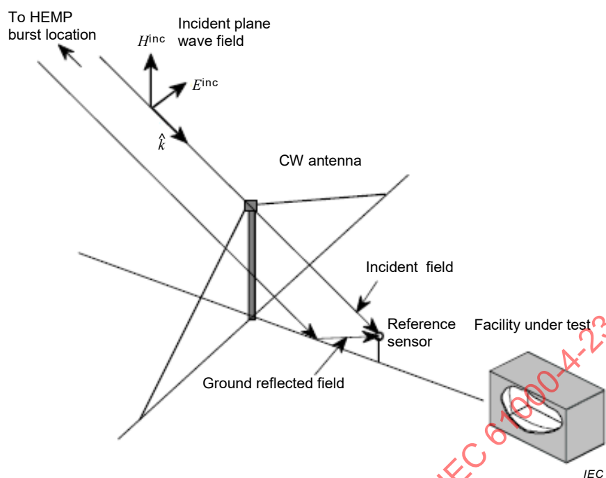
Figure D.3 – Incident and ground-reflected field contributions to the reference sensor excitations
