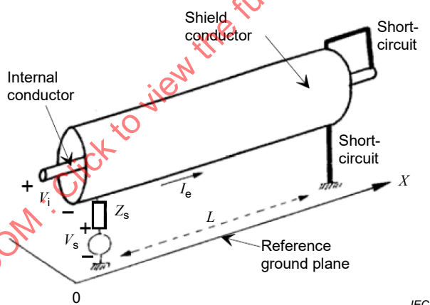
Figure 8 – Basic configuration for transfer impedance measurement
