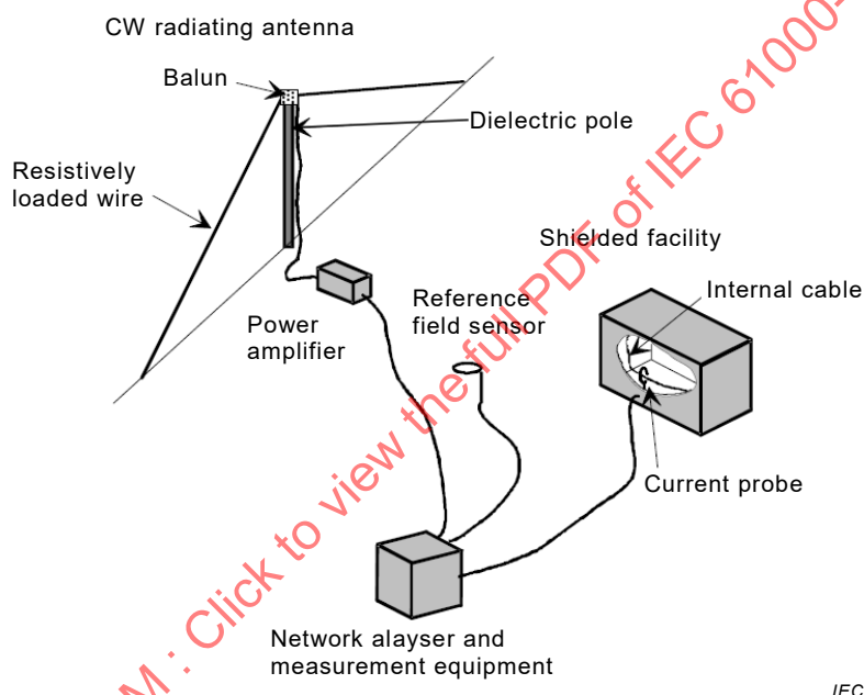
Figure 21 – Typical configuration of a CW test facility
