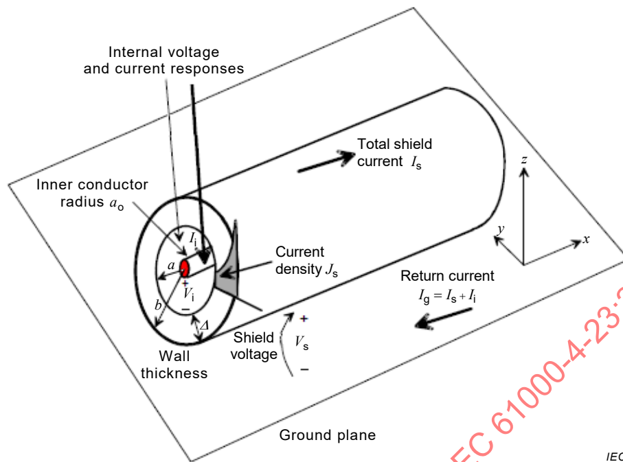
Figure B.2 – Coaxial cable located over a conducting ground plane
