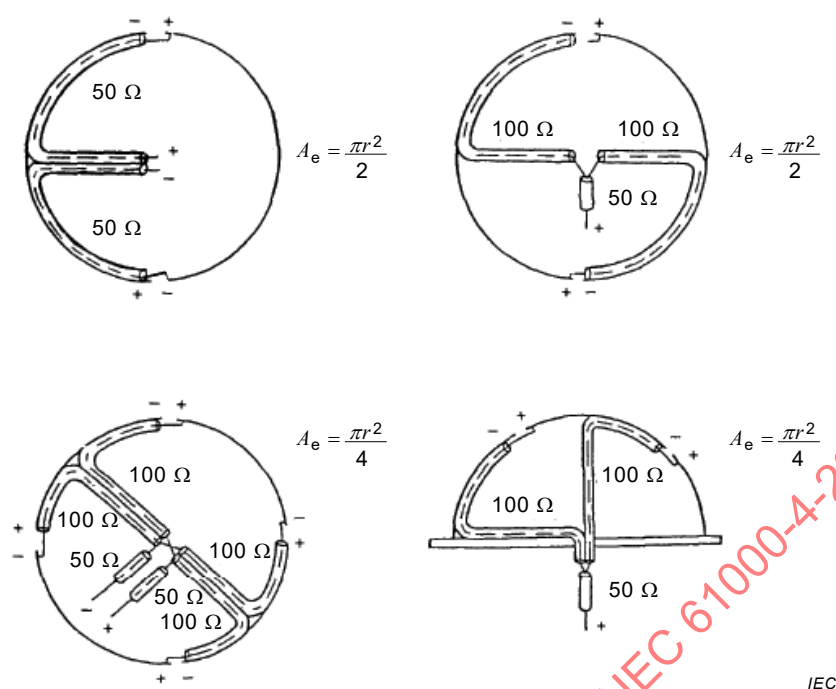
Figure C.3 – Two- and four-slot cylindrical coil sensors [23]
