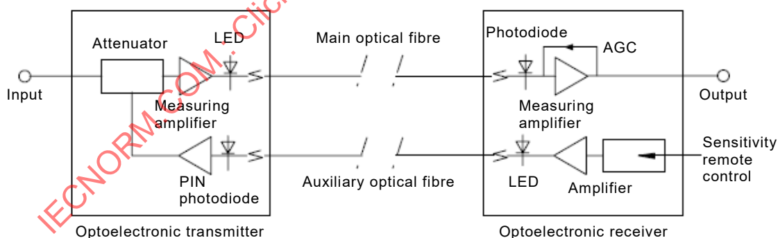
Figure C.11 – Example of a single-channel fibre optic transmission system [23]
