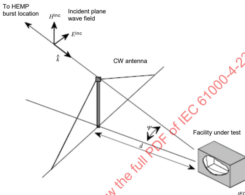
Figure D.2 – Relationship between the CW antenna and the incident HEMP field
