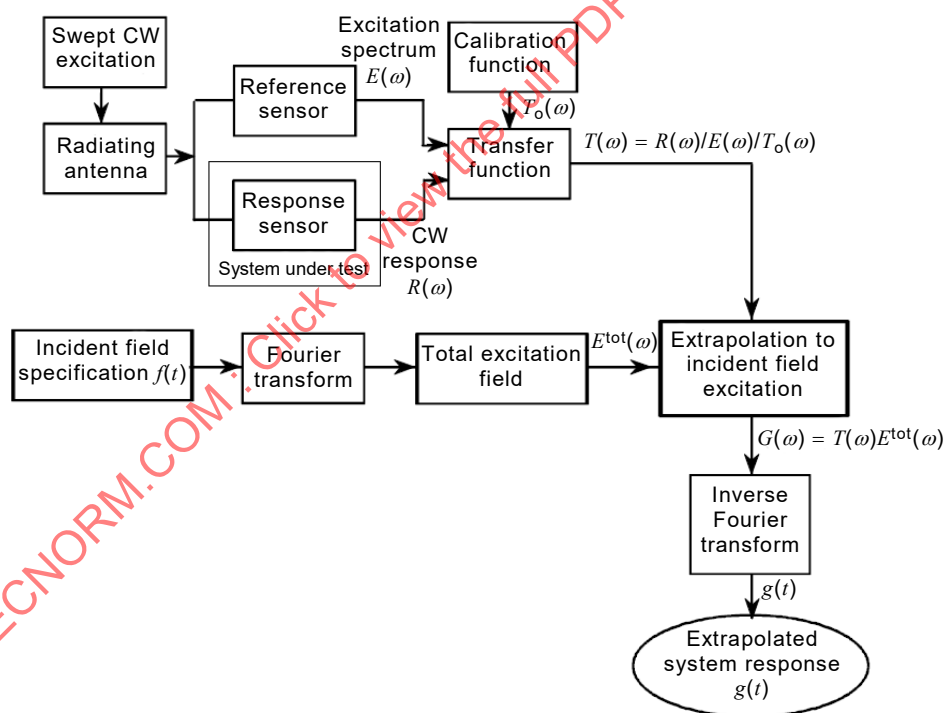
Figure 24 – Analysis flow diagram for extrapolating a measured CW spectrum to the HEMP response
