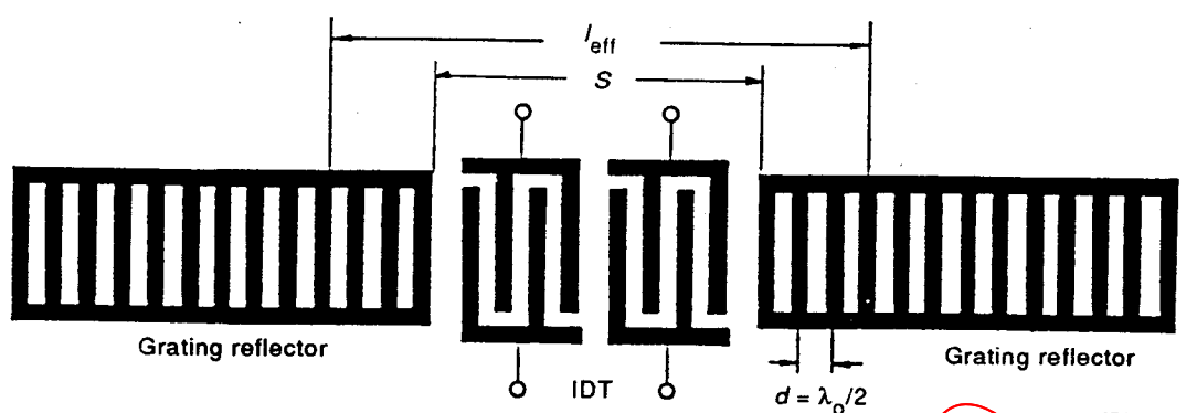
Figure 2 – Two-port SAW resonator configuration
