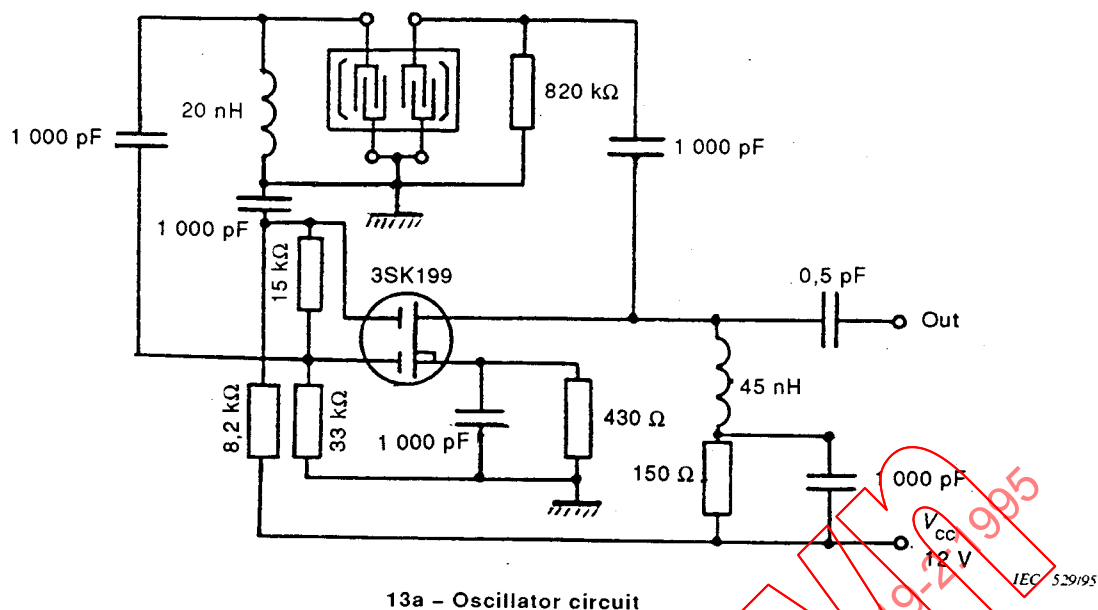
13a - Oscillator circuit
