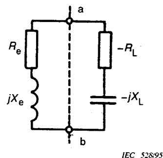
12c – Equivalent circuit
