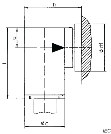
Figure 18c) – Housing variant 3
