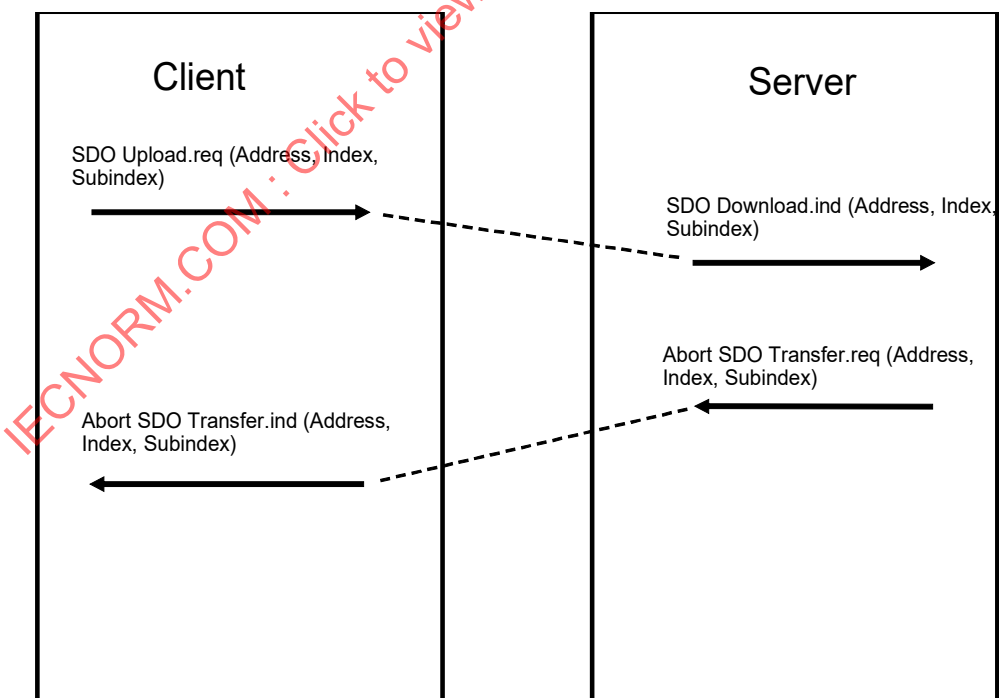
Figure 15 – Unsuccessful single SDO-Upload sequence
