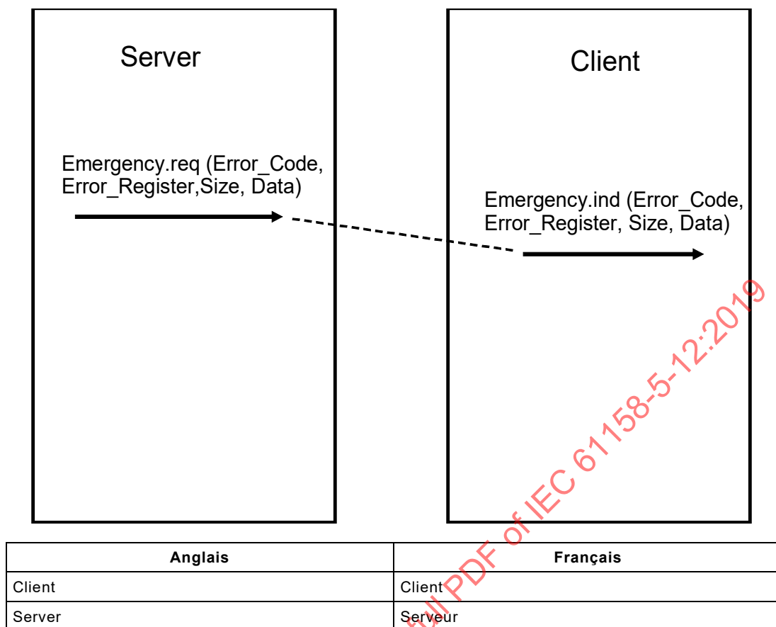
Figure 18 – Service 'Emergency' (Urgence)
