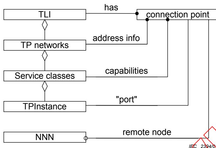
Figure 2 – Relationship between TLI, TP networks and ports
