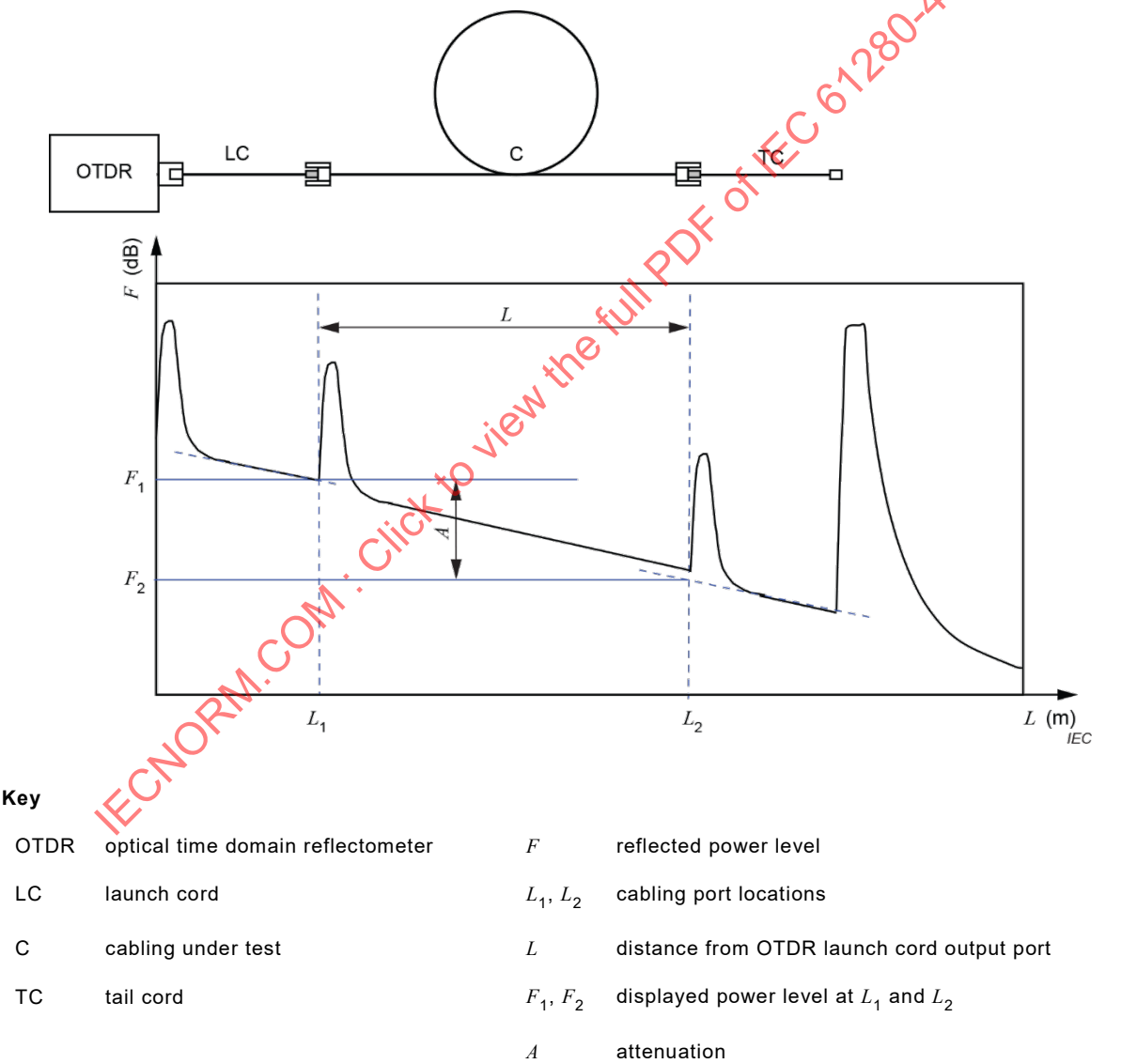
Figure E.3 – Graphic construction of F_1 and F_2
