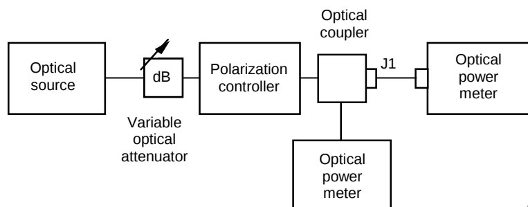
Figure 1a - Input signal power measurement
