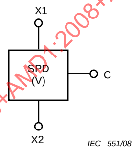
Figure 1c – Three-terminal SPD
