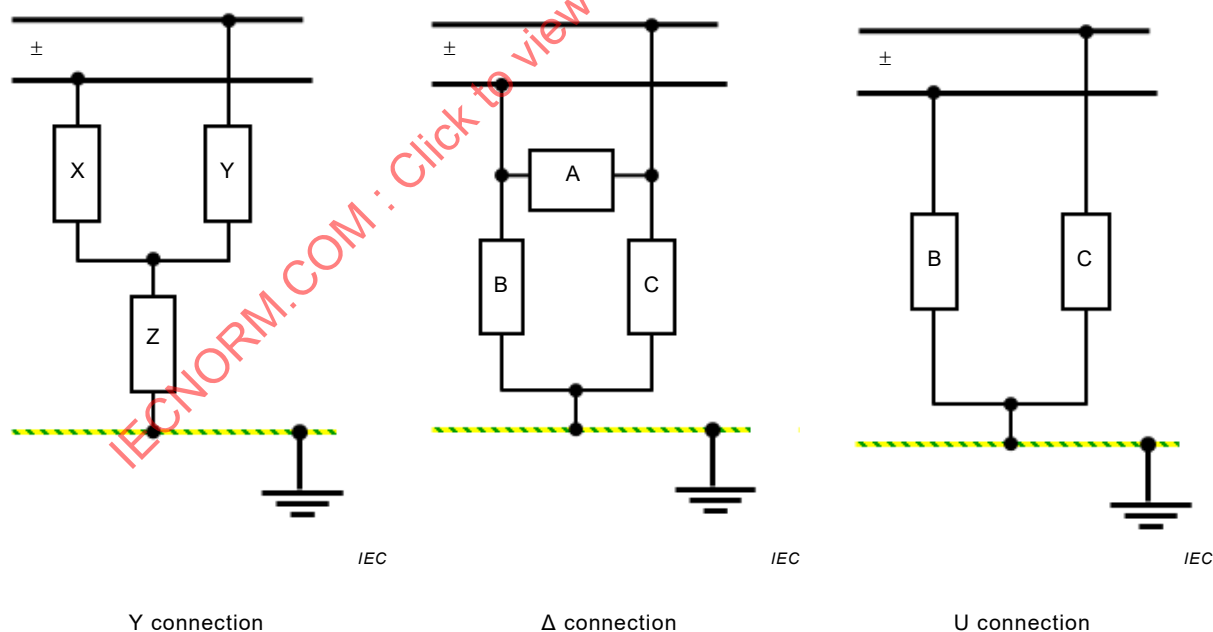
Figure 7 – Example of SPD connections on the DC side of an unearthed PV source
