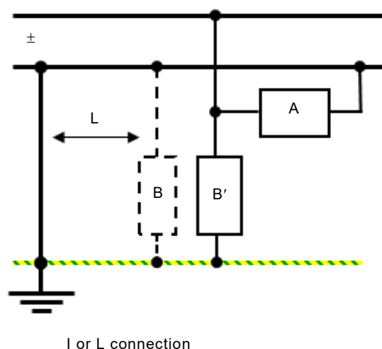
Figure 8 – Example of SPD connection on the DC side of a reliable earthed PV source
