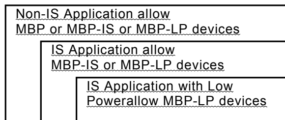
Figure 3 – CP 3/2 Slave devices usable in applications
