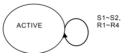
Figure 14 – State transfer figure of periodic data transmission
